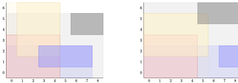
Figure 1: The algorithms to be tested in samples 1 and 2, respectively. The boxes indicate the parameters where an algorithm must be tested, while the lighter background indicates the region where an algorithm can be used to verify other algorithms.
