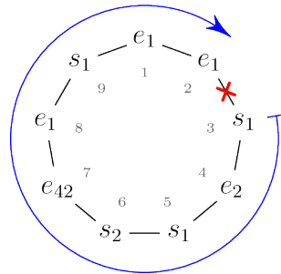
Figure 1: Illustration of Sample Input 1 with its optimal cutting location.
